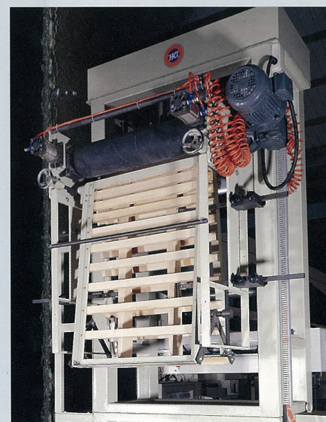
COLLAPSING FRAME/MAIN PINCH ROLLERS/GUESSETING DEVICE
