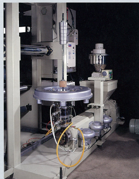
EXTRUDER/DIE HEAD/AIR RING/STABILIZER
